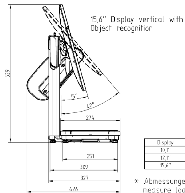
Q1_expert_800_side_view_15,6_display_vertical_object_recognition
