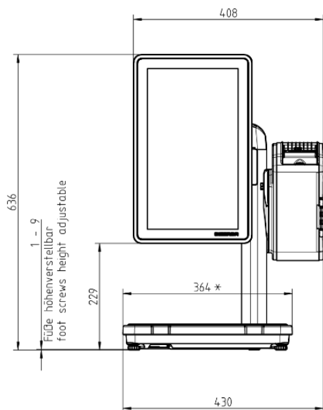
Q1_expert_800_front_view_vertical
