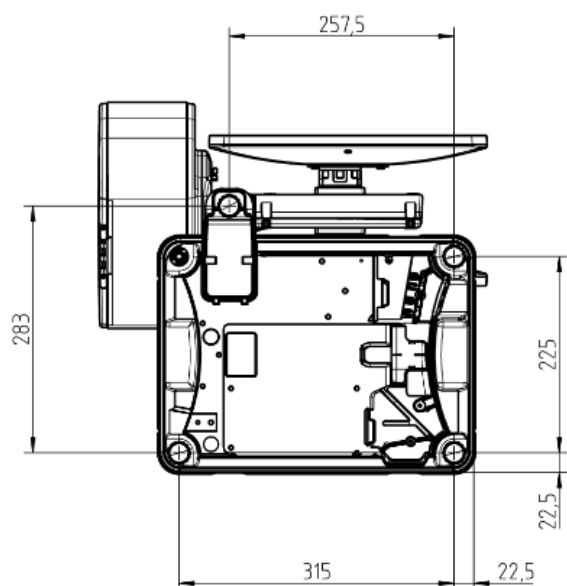
Q1_expert_800_view_from_below
